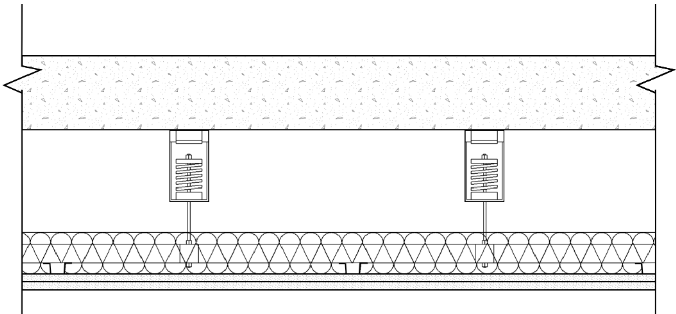
Figure 8 Cross section of A1-019524-05F.
