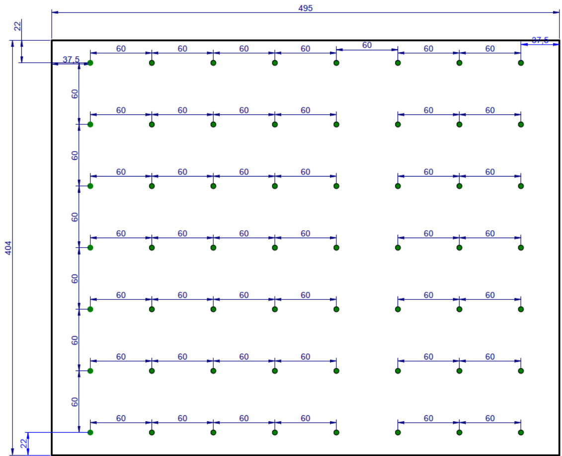
Figure 4 Floor mount installation layout.
