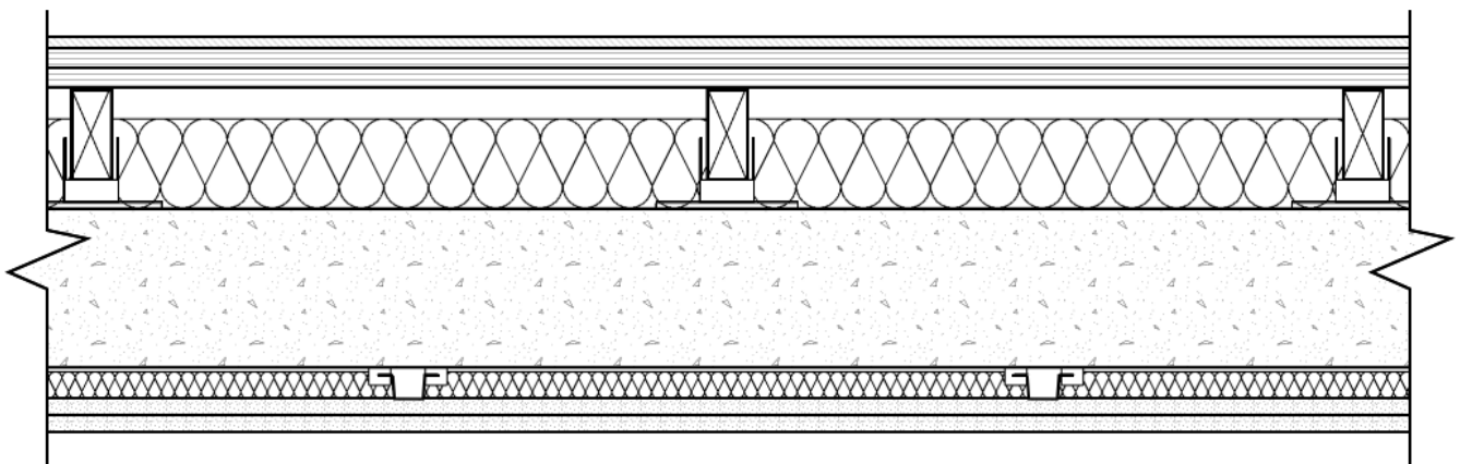
Figure 3 Cross section of A1-019524-02F.
