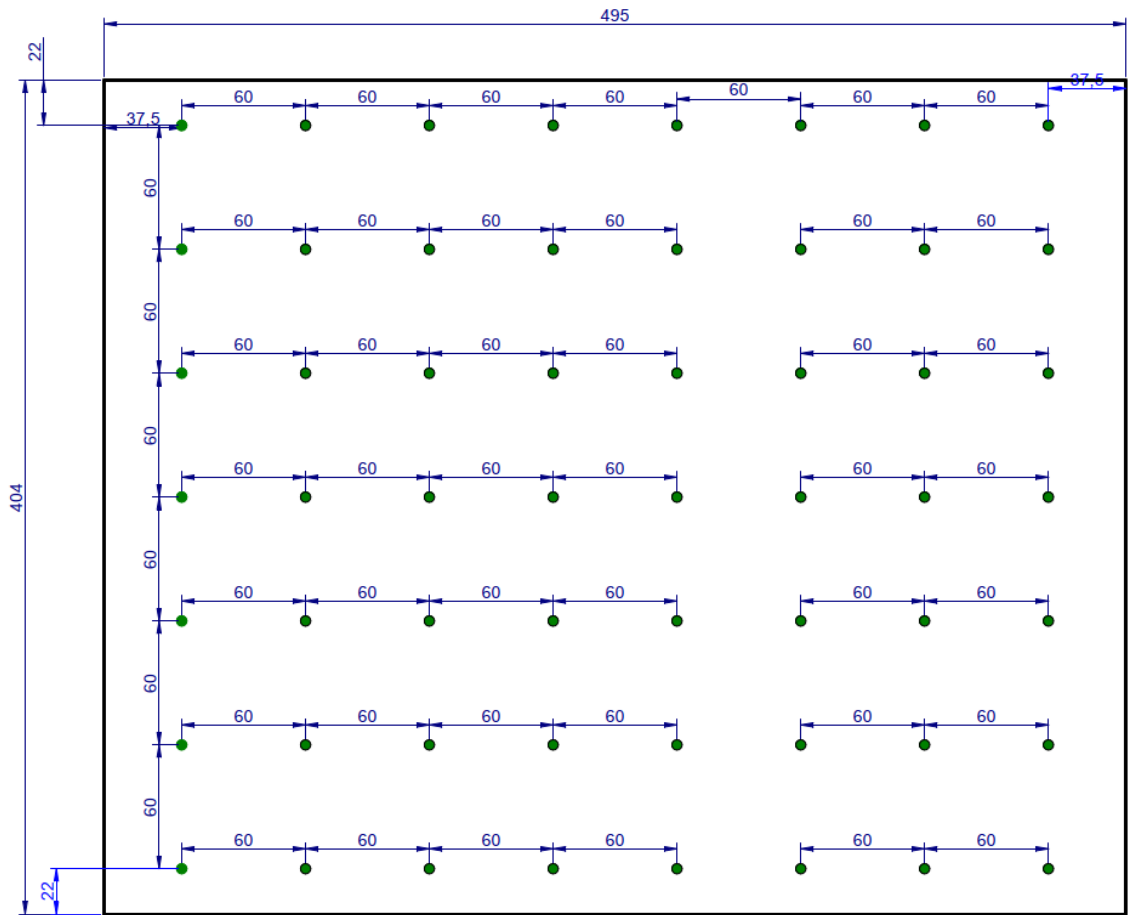
Figure 2 Floor mount installation layout.
