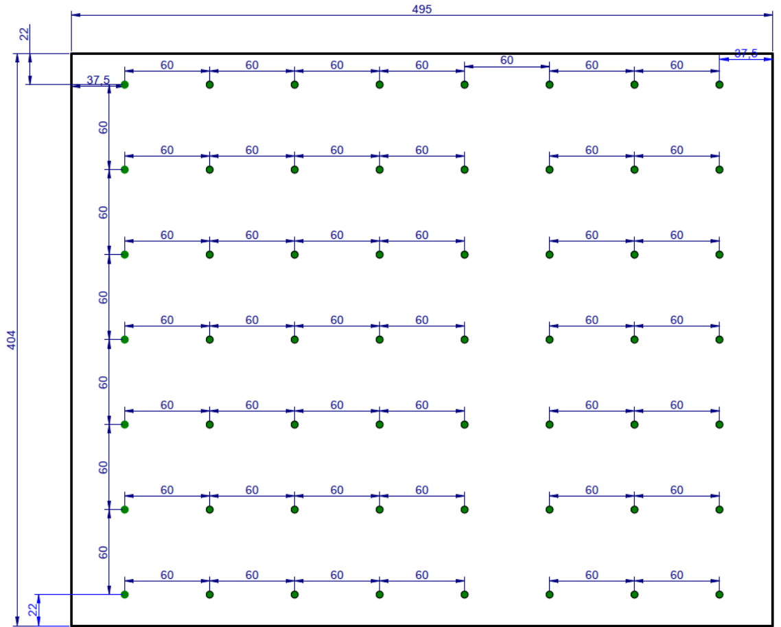
Figure 6 Floor mount installation layout.
