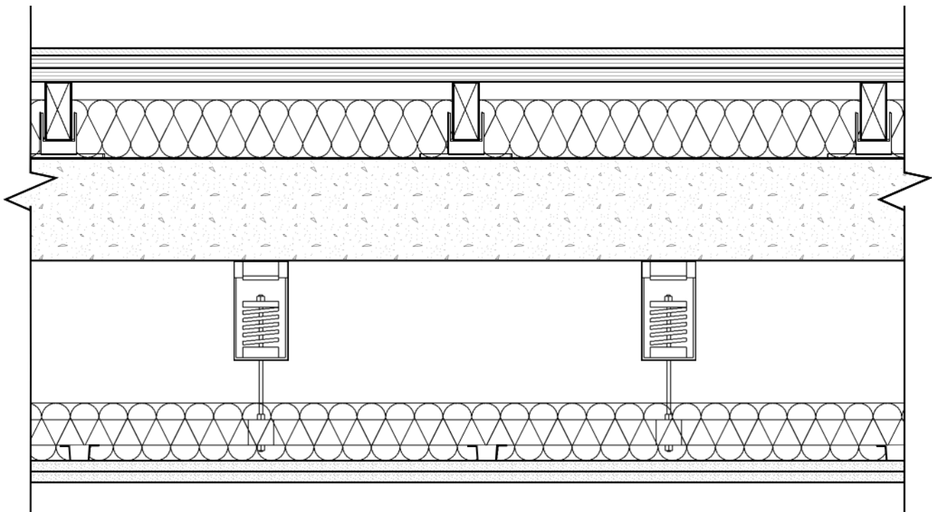
Figure 7 Cross section of A1-019524-04F.
